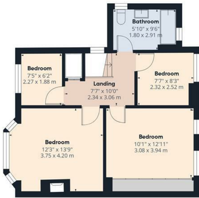
Floor 1 Building 1
