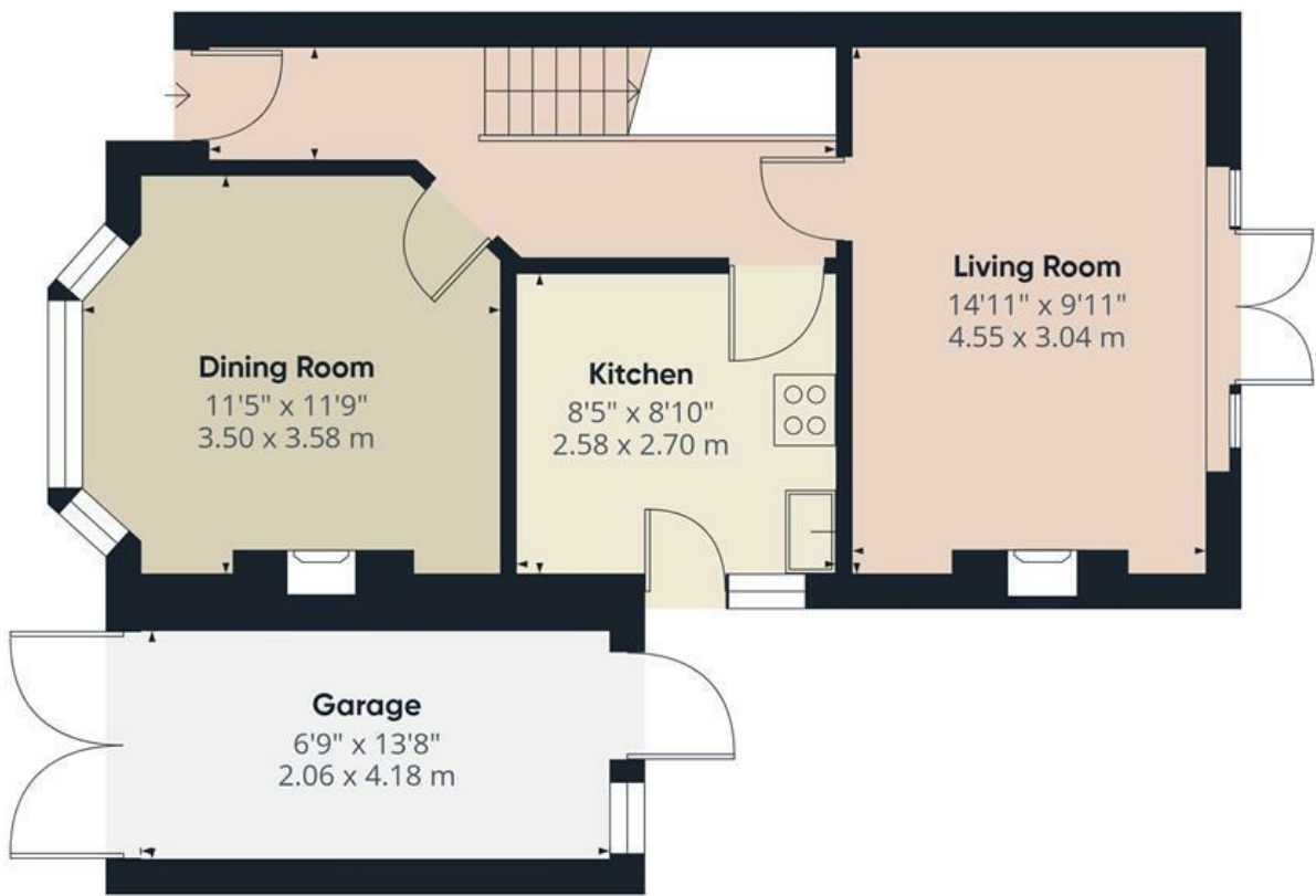
Ground Floor Building 1
